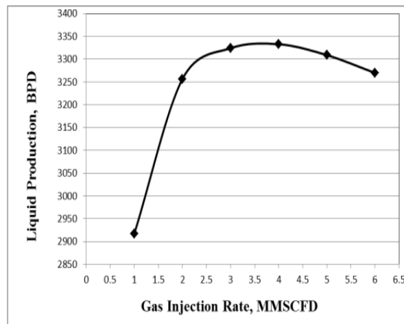
Fig 3.. Basic characteristics of well A.
