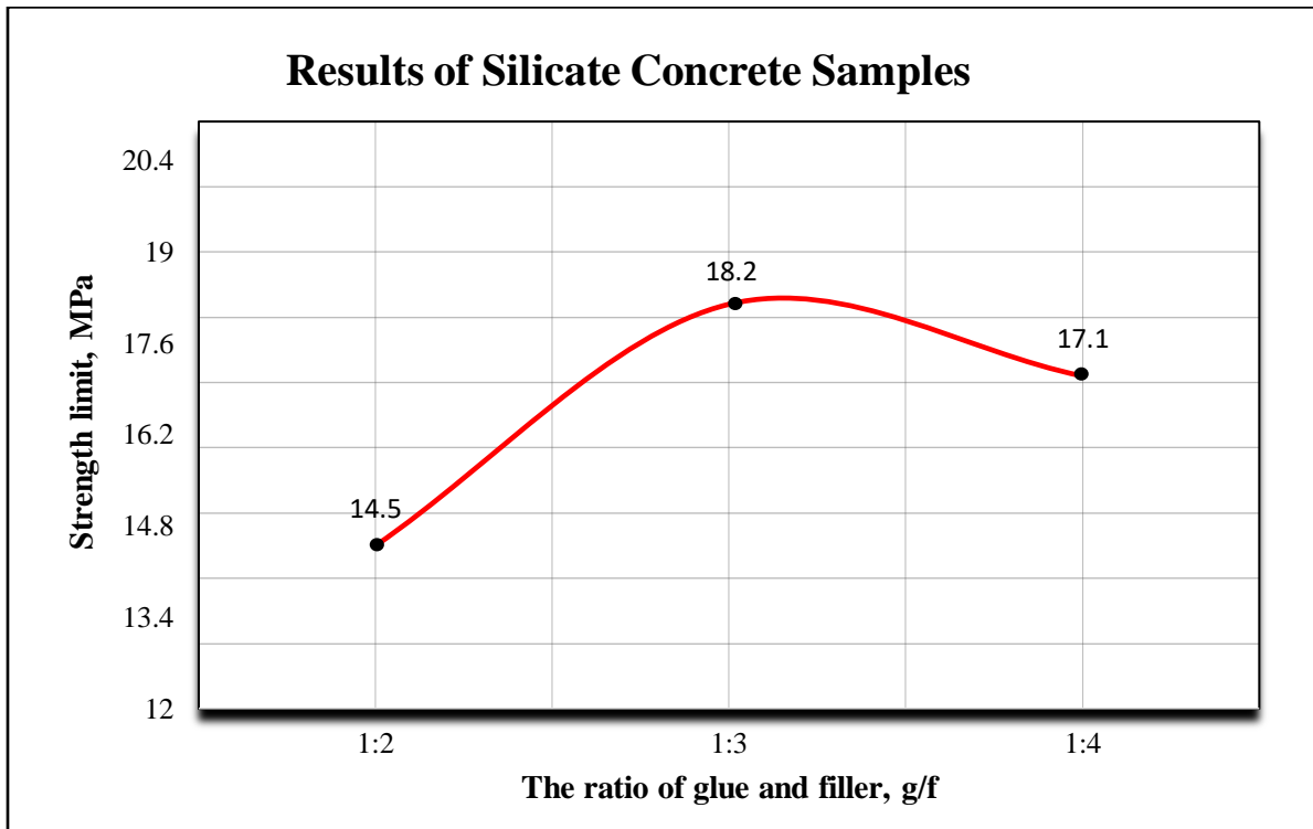
Figure 2. Results of silicate concrete samples
