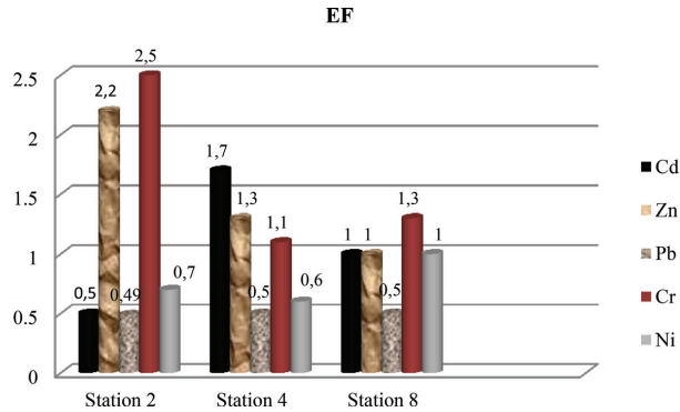
01 Figure 3. Change of the values of enrichment factor of heavy metals in the grounds of three study stations.
