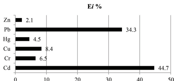
02 Figure 8. Percentage of heavy metals in potential ecological risk (RI) for the sediments of Bulbula Lake.
