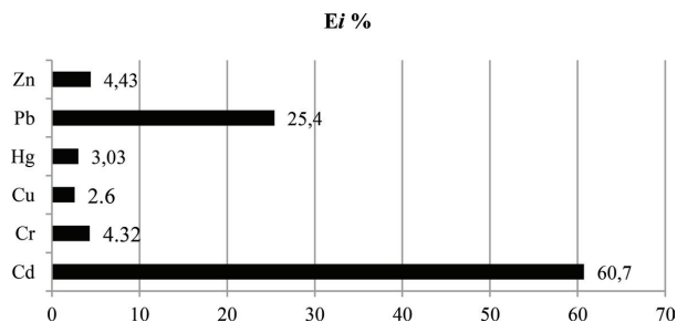
01 Figure 7. Percentage of heavy metals in potential ecological risk (RI) for the sediments of Boyuk shore Lake.
