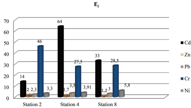
02 Figure 4. Change of the values of potential ecological risk index of heavy metals in the grounds of three study stations.
